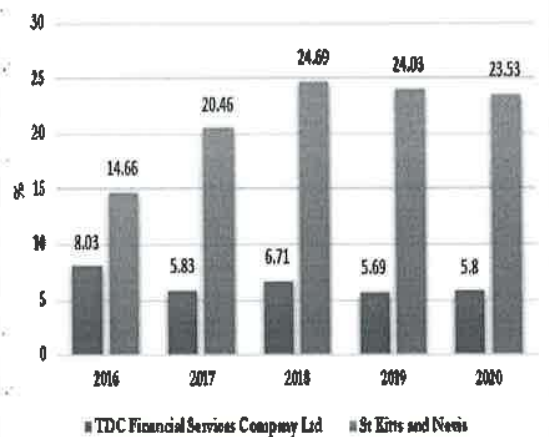
Delinquency Rates
